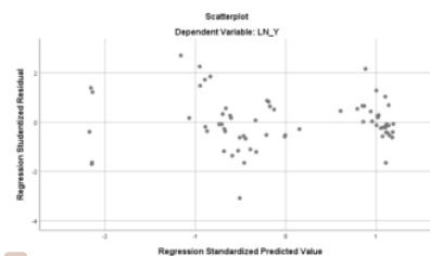
7 Figure 2. Heteroscedasticity Test Results
