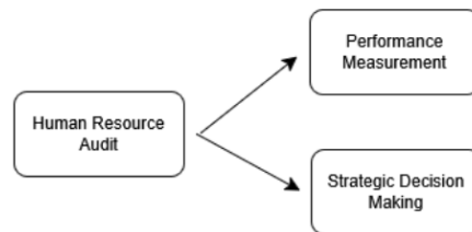
Fig 1. Research Conceptual
